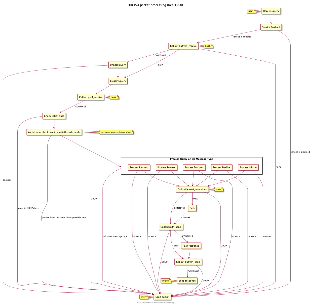
Fig. 2: DHCPv4 packet processing
